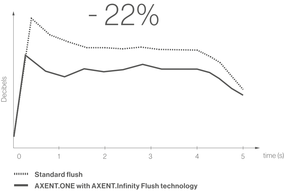
Maximum decibel level of flush noise
