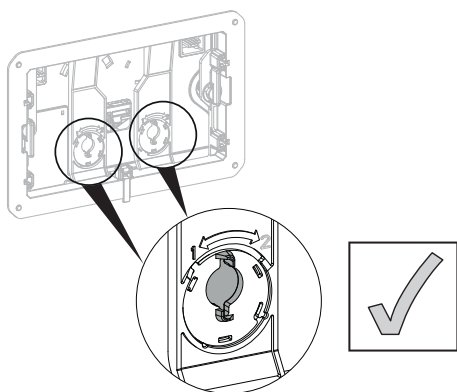
AXENT concealed cistern K133, K212, K310
